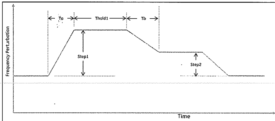
Figure 3.1.1d: Test Injection Signal Form 4
