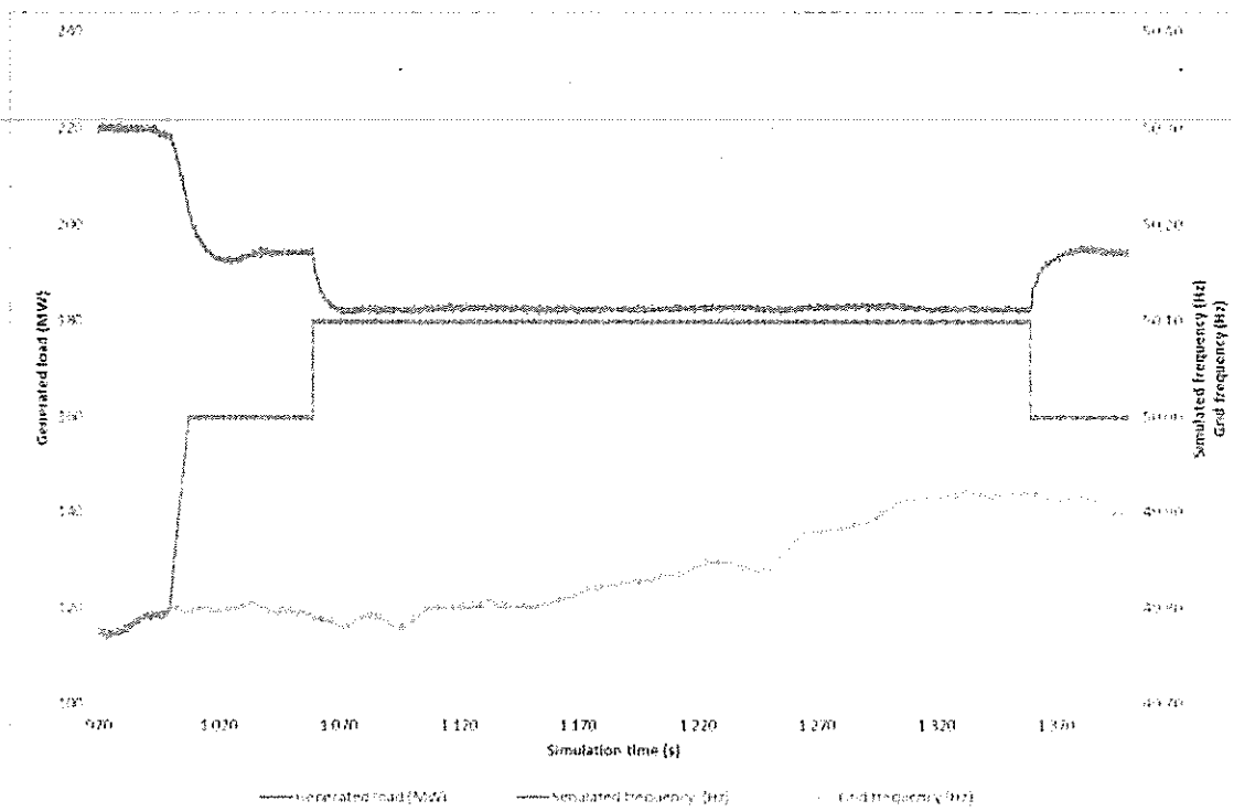
Figure 7: Frequency steps in FGMO, generated load 90 %, droop 4%, Part 2
